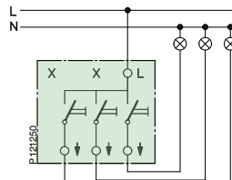
3 x 1-pol
