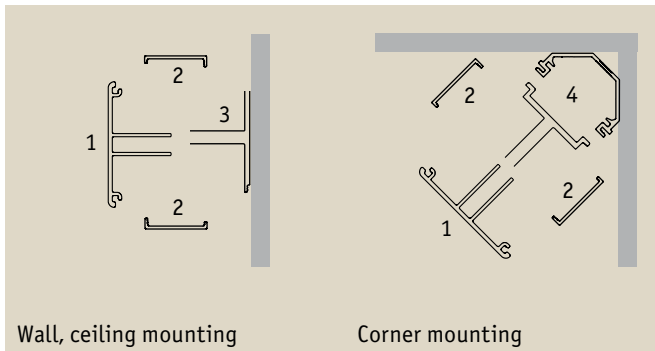
Flat strip light without diffuser
