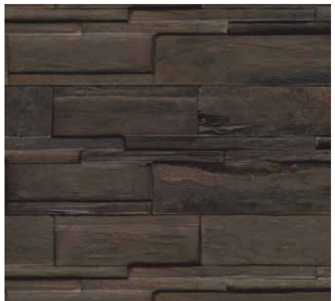
SULU SEA
