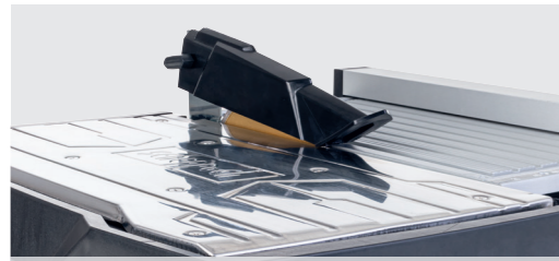
The protective cover can be height-adjusted, different material thicknesses can therefore be cut safely.
