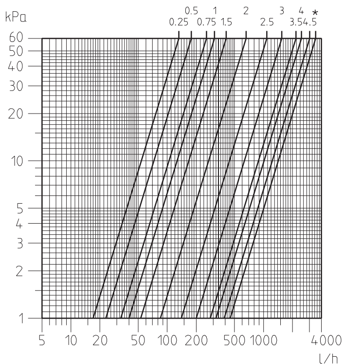
Diagram DN 20 (1") – PN 16 (50 007)
