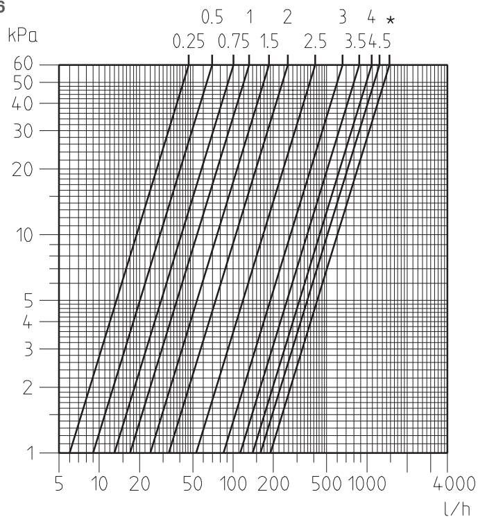
Diagram DN 15 (1/2") – PN 16 (50 007)
