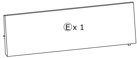
Backrest Right 1670x500x100 mm
