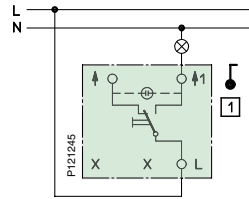
Trapp/1-pol
