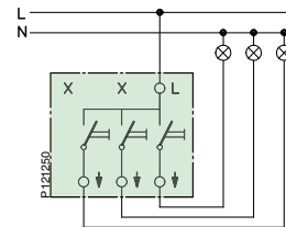
3 x 1-pol
