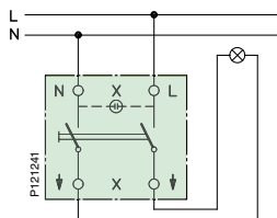
2-pol
