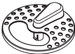
D x2
